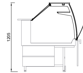
VCV VCV - Vidro convexo / Convex glass / Vitrage convexe
